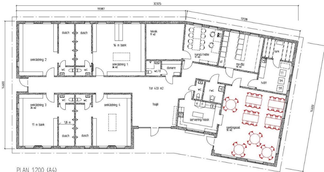
PLAN 1:200 (A4)
